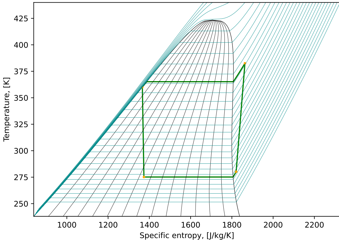
Conceptual HP Cycle - R1234ze(Z)
